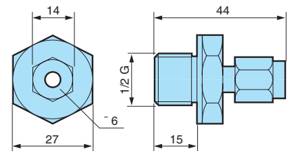
Connection: 79696040
