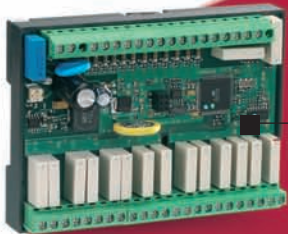
Millenium 3 expanded bare board with 16 relay outputs
