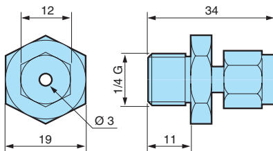
Connection: 79696038
