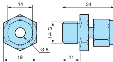
Connection: 79696039
